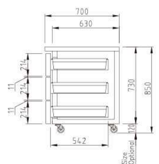
SIDE VIEW (Depth 700mm)
