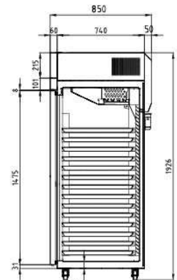
SIDE VIEW LONG DOOR
