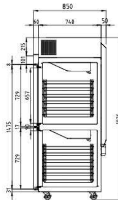
SIDE VIEW KRF25-2P
