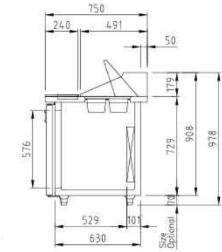
SIDE VIEW (Depth 750mm)
