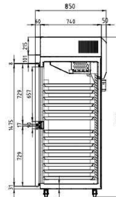
SIDE VIEW HALF DOOR
