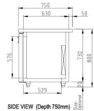
SIDE VIEW (Depth 750mm)
